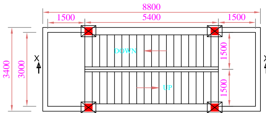
TYPICAL PLAN
